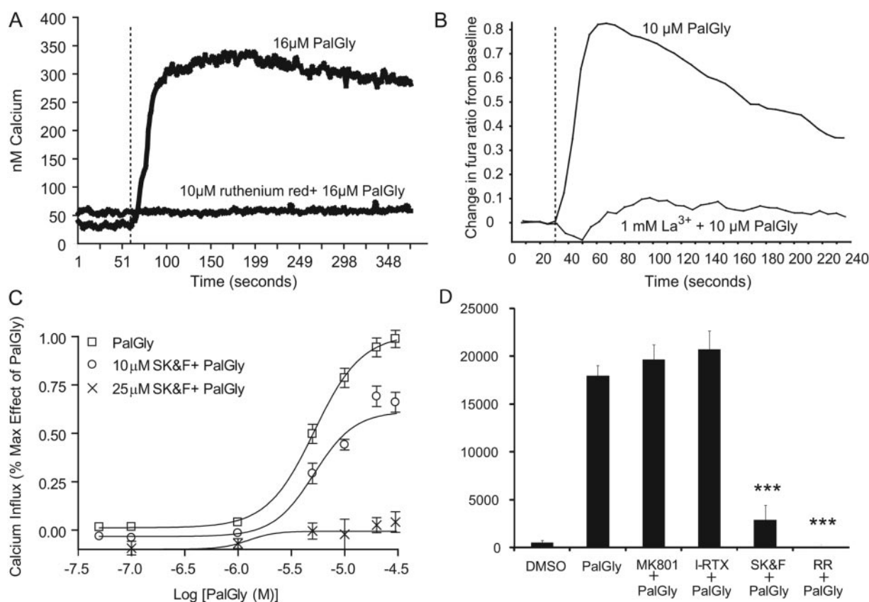
Fig. 6. PalGly-induced calcium influx was inhibited by pretreatment with ruthenium red (10 \mu M), SK&F96365 (25 \mu M), and La 3+ (1 mM). A, single cell calcium traces for F-11 cells treated with 16 \mu M PalGly after administration of vehicle or 10 \mu M ruthenium red. B, a representative F-11 well population calcium influx of cells pretreated with La 3+ or vehicle. C, concentration-response curves for PalGly and PalGly + SK&F96365 (10 or 25 \mu M) show profound inhibition of PalGly-induced calcium influx in F-11 cells after treatment with 25 \mu M SK&F96365. n = 3–20 wells per condition. D, PalGly (16 \mu M) induced marked calcium influx in the presence of MK801 (25 \mu M) and I-RTX (35 nM), whereas it lacked efficacy in the presence of SK&F96365 (10 and 24 \mu M) or ruthenium red (10 \mu M). Calcium mobilization was calculated from the integral of the calcium concentration \times time curve as described in the text. ***, p < 0.001 difference from vehicle + PalGly. One-way ANOVA with LSD post hoc tests. Error bars indicate S.E.M.
